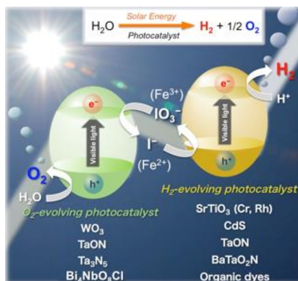
Fig. 1 Conceptual scheme for photocatalytic water splitting under visible light through two-step photoexcitation.
